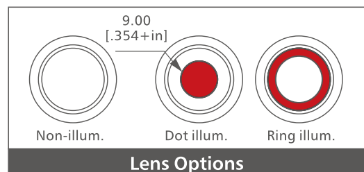
Panel Cutout
